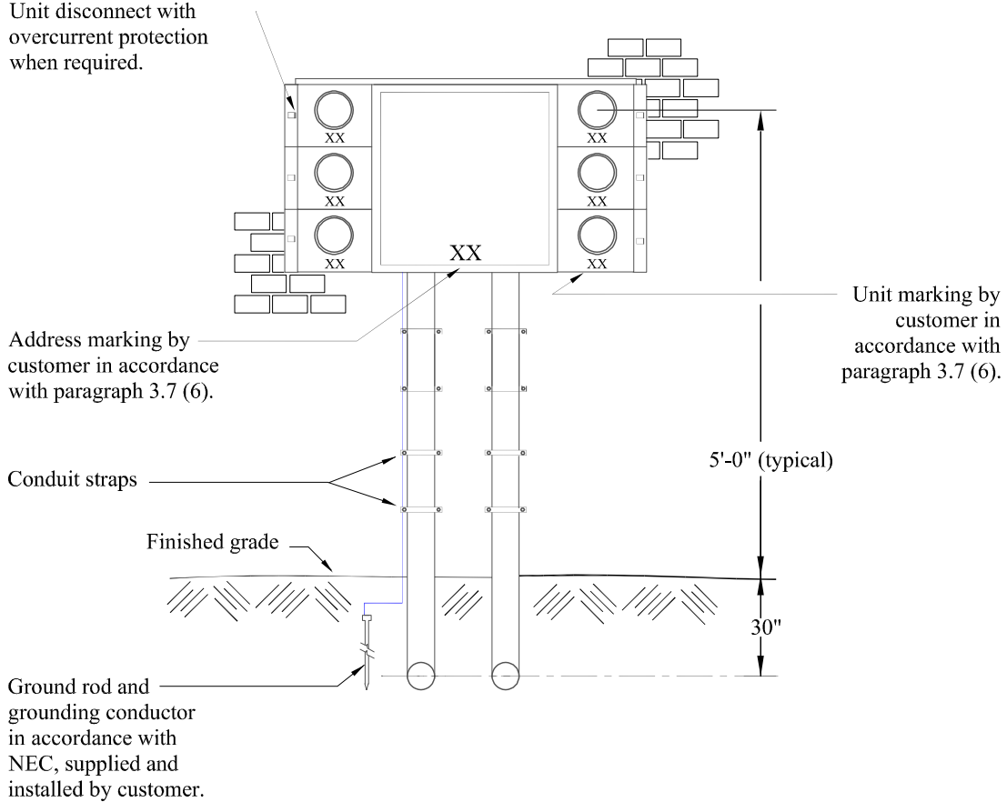
Customer Owned Meter Center Two to Six Positions
